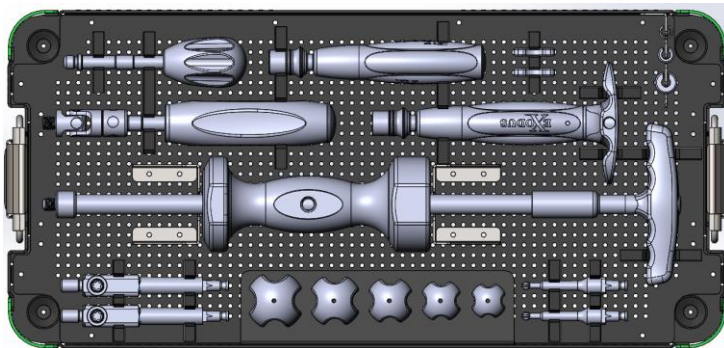
HANDLE TRAY
