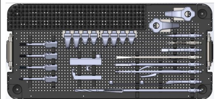
ATTACHMENT TRAY
